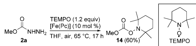
Scheme 4. Reaction of methyl carbazate ( 2a ) and TEMPO.
